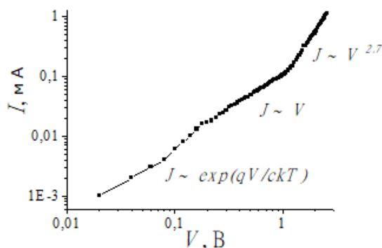
Fig.1. Direct branch of the current-voltage characteristic of the p-Si-n-(Si 2 ) 1-x (GaN) x structure in logarithmic scales.
